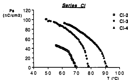
Figure 3. Temperature dependence of the polarization of the compounds in series Cl (Cl-2, Cl-3, and Cl-4) in the SmC* phase.
